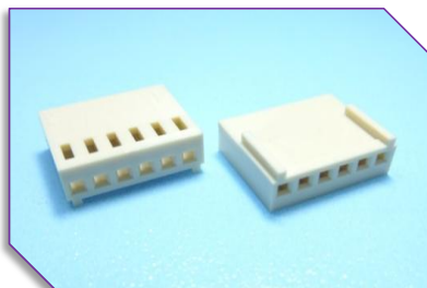
E24 2.54mm Housing
