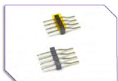
B30S 1.27mm Pin Header SMT + R/A
