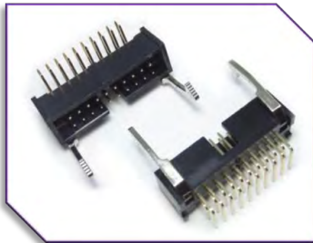
F22L 2.54mm Box Header with Metal Latch
